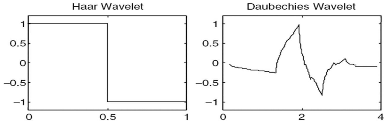
Figure 10.27 The general shape of two wavelets commonly used in wavelet analysis. The sharp corners enable the transform to match up with local details that cannot be observed when using a Fourier transform that matches only sinusoidal shapes.
